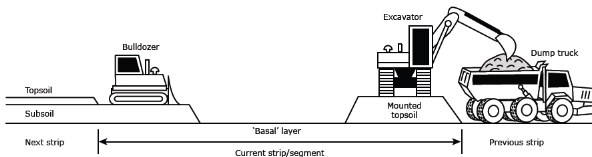
Figure I.3: Soil stripping with bulldozers and dump trucks using modified layer by layer method: Subsoil.
